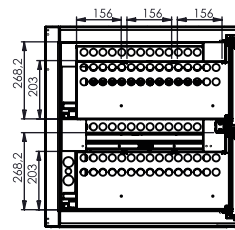
SOCKET 1/2
