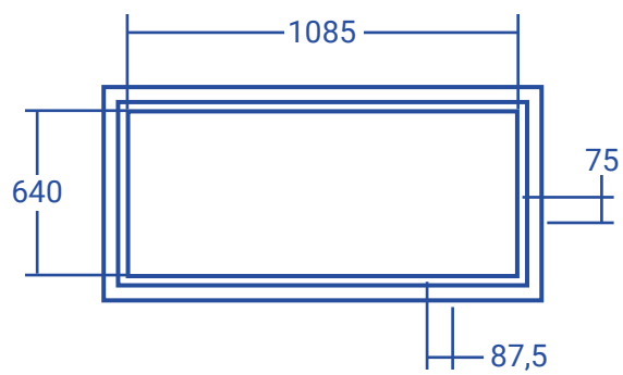
Top view the glass-ceramic plate
